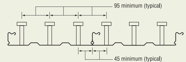
10 studs/metre (single row) – nominal 100 spacing
